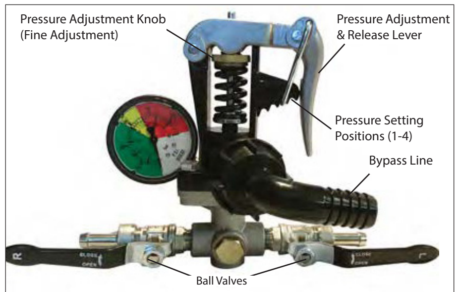
Figure 1: Operator Controls
