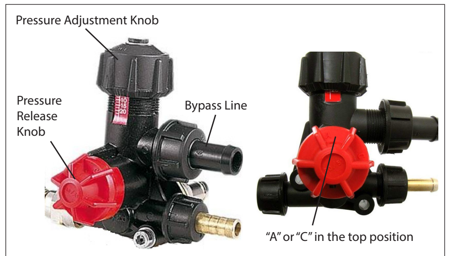
Figure 2: Operator Controls
